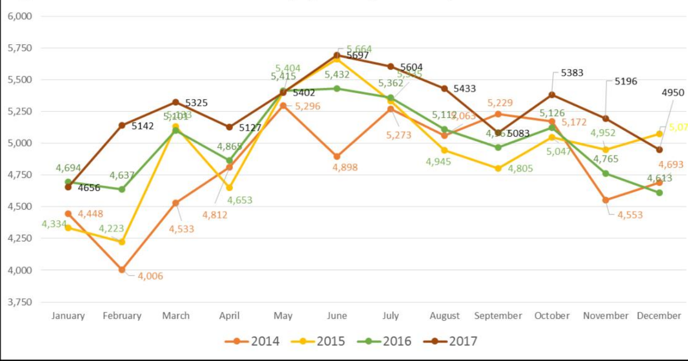
Figure 5. McLean Station Calls for Service, by Month (2014-2017)
