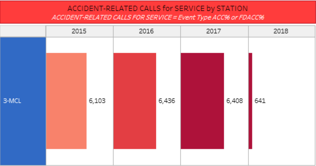
Total calls for accidents (reportable and non-reportable)
