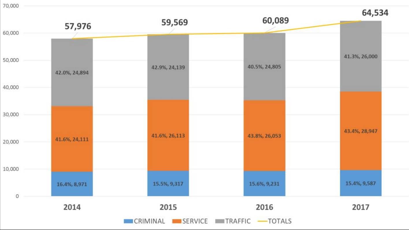
Figure 4. MCLEAN STATION CALLS FOR SERVICE, by TYPE (2014-2017)
