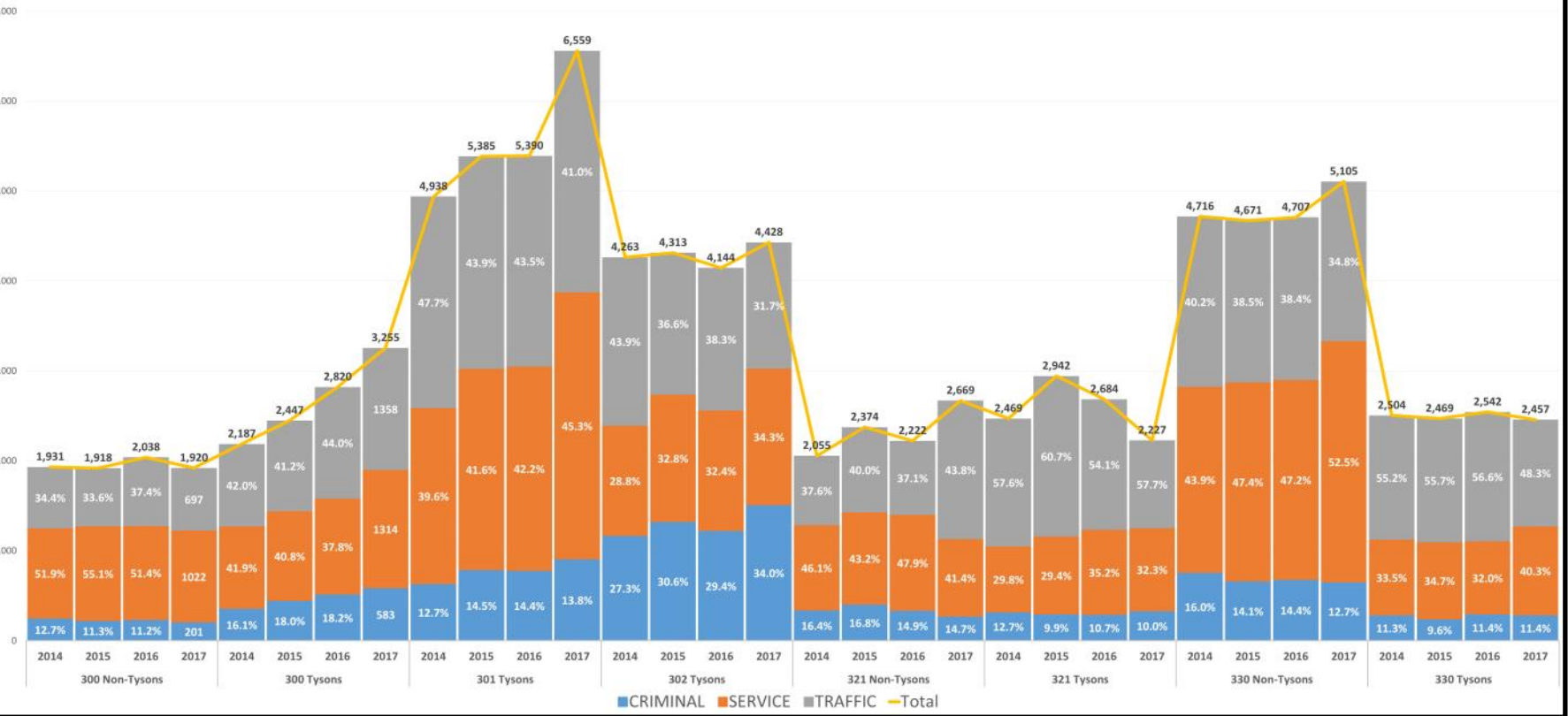
Figure 7. Estimated Calls for Service by Patrol Areas of Tysons, by Portions Inside and Outside of the Designated Urban Area, by Type (2014-2017)
