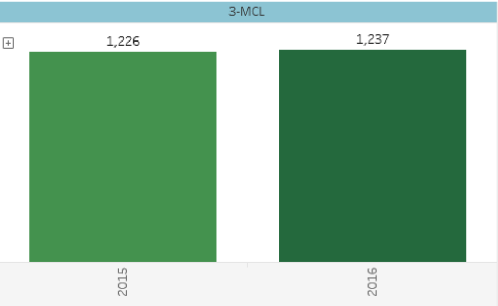
TOTAL REPORTABLE CRASHES by ADDRESS (SORTED BY DESCENDING 3-YEAR TOTAL)
